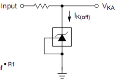
Test Circuit for I_{K(\text{off})}
