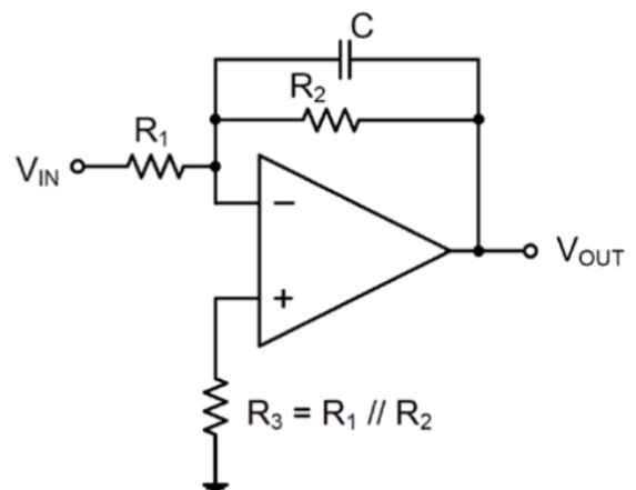
Figure 6. Low Pass Active Filter
