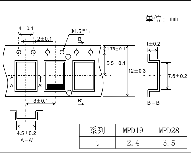
编带 Carrier Tape
