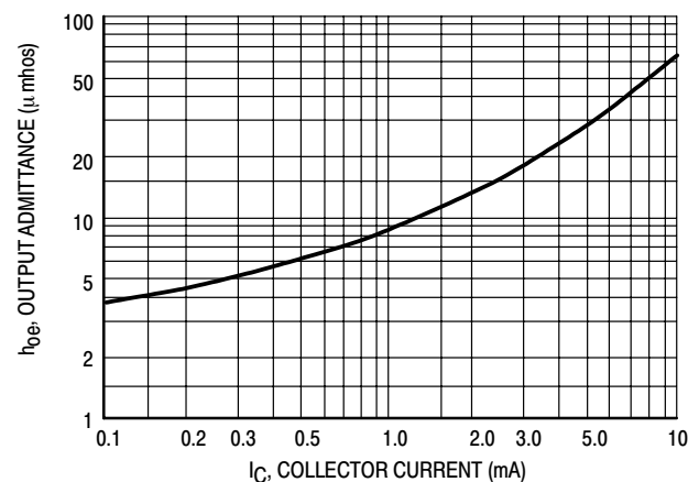
Figure 10. Output Admittance
