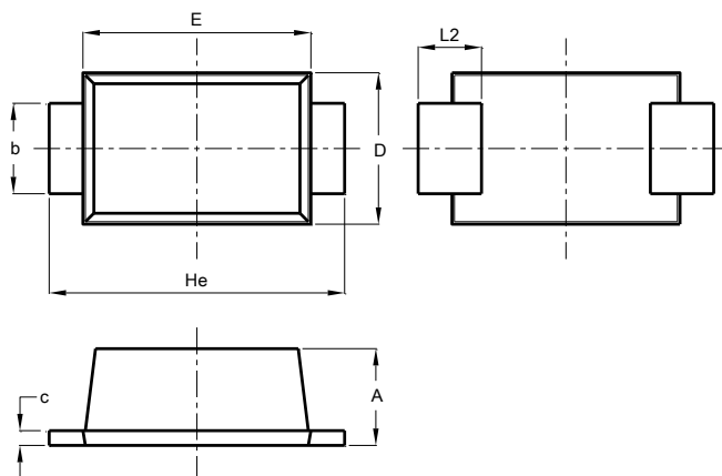
SOD123FL
