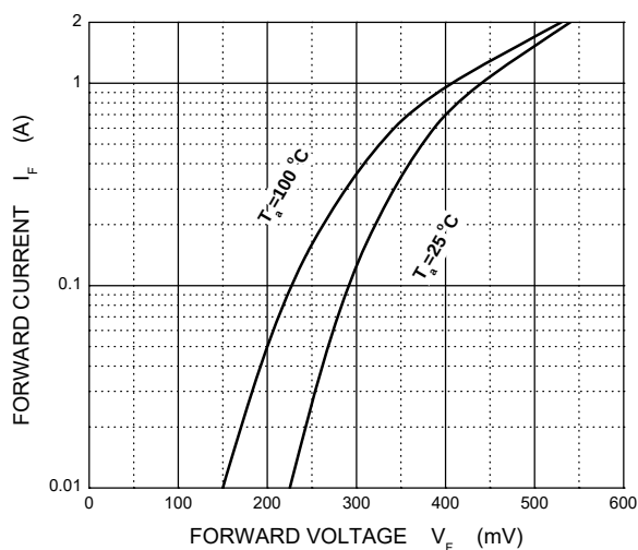
FIG.2-TYPICAL FORWARD CHARACTERISTICS
