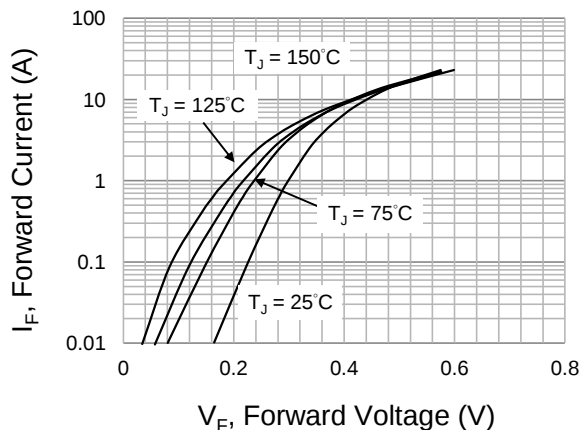
FIG.2-TYPICAL FORWARD CHARACTERISTICS
