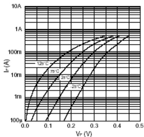
FIG.2-TYPICAL FORWARD CHARACTERISTICS
