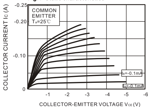
Fig.1 Static characteristics
