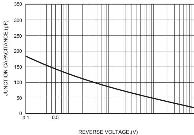
FIG.6-TYPICAL JUNCTION CAPACITANCE
