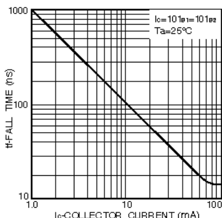
Fig.11 Fall time vs. collector current
