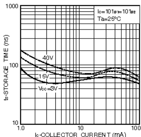
Fig.10 Storage time vs. collector current
