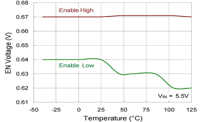
Enable Threshold vs. Temperature
