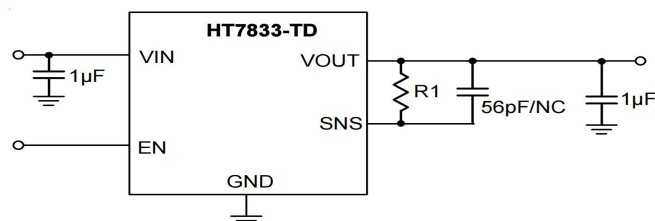
Figure 5. Fine Adjustable Output Voltage Application Circuit
