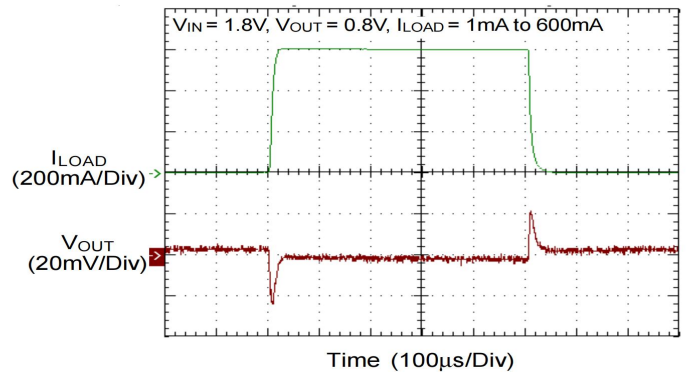
Load Transient
