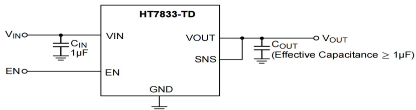
Figure 1. Application with Sense Function
