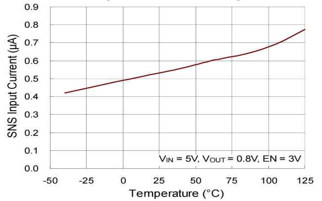
SNS Input Current vs. Temperature
