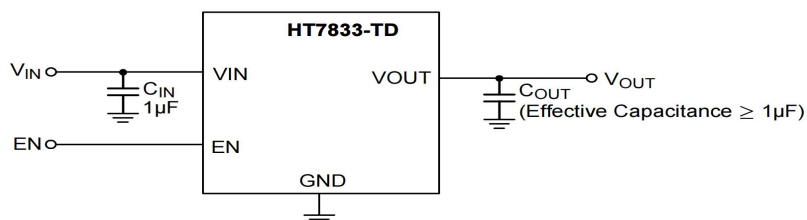
Figure 2. Application without Sense Function
