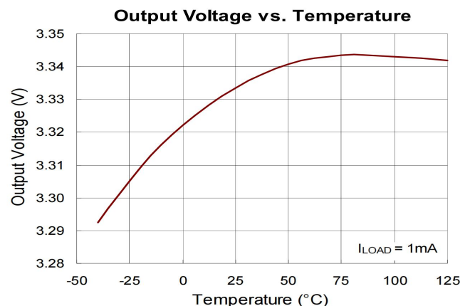
Figure 4. Temperature Coefficient of Adjustable Output Voltage
