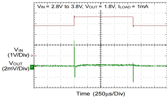
Line Transient
