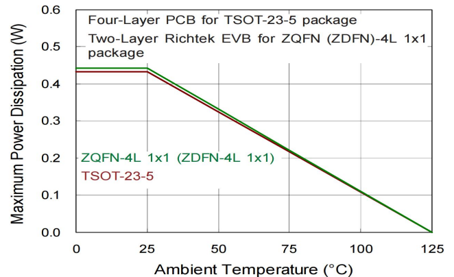
Figure 6. Derating Curve of Maximum Power Dissipation
