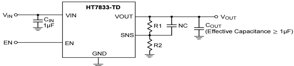
Figure 3. Adjustable Output Voltage Application Circuit
