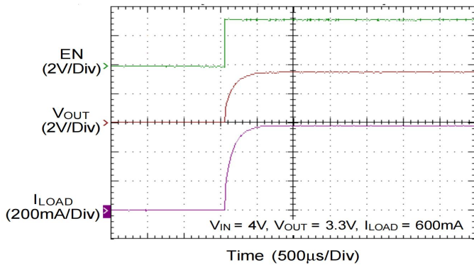
Power On from EN
