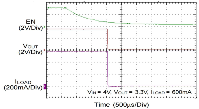
Power Off from EN
