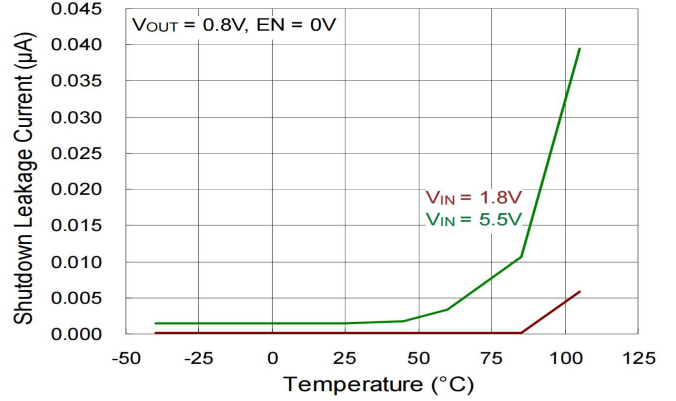
Shutdown Leakage Current vs. Temperature
