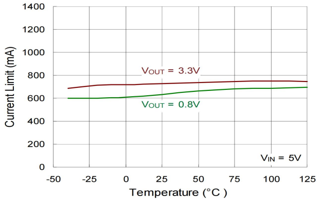
Fold-Back Current Limit vs. Temperature
