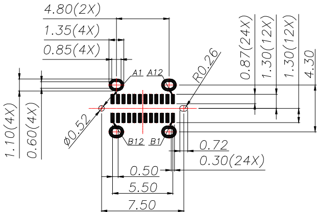
RECOMMENDED P.C.B. LAYOUT(24 Pin)
