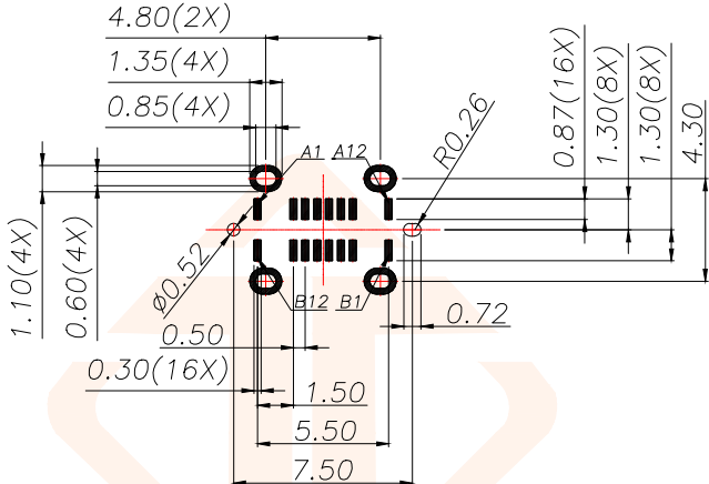
RECOMMENDED P.C.B. LAYOUT(16 Pin)
