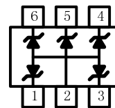
Pin Configuration
