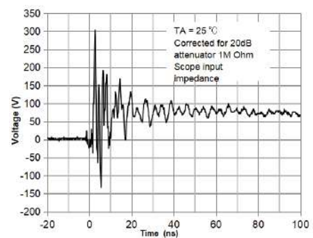
TLP Curve
