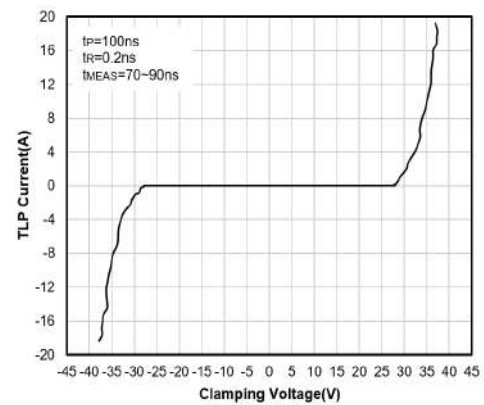
TLP Curve
