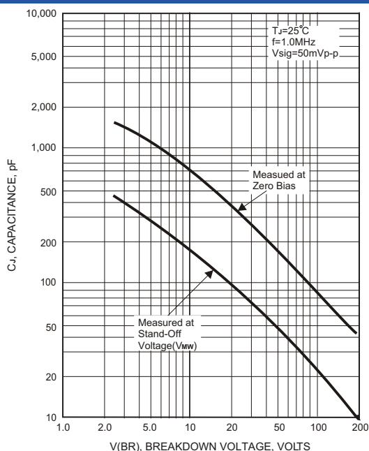
FIG.5-TYPICAL JUNCTION CAPACITANCE
