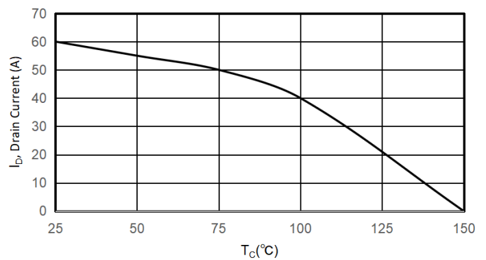
Figure 10: Maximum Continuous Drain Current vs. Case Temperature
