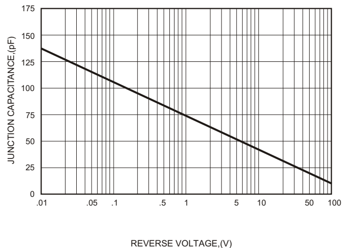
FIG.6-TYPICAL JUNCTION CAPACITANCE
