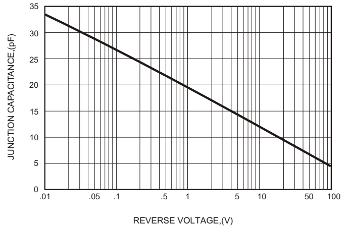
FIG.6-TYPICAL JUNCTION CAPACITANCE
