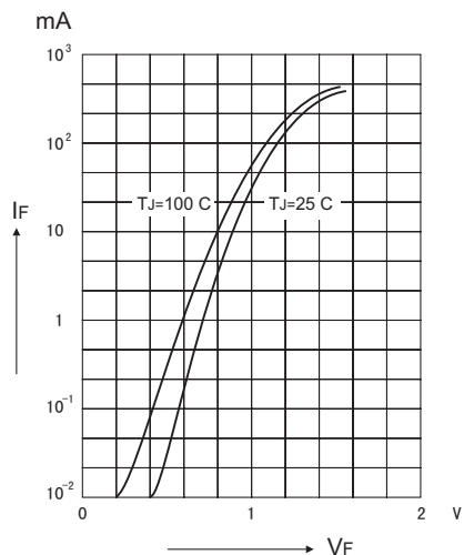
FIG.1-TYPICAL FORWARD CHARACTERISTICS
