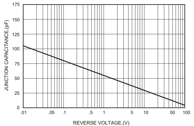
FIG.6-TYPICAL JUNCTION CAPACITANCE
