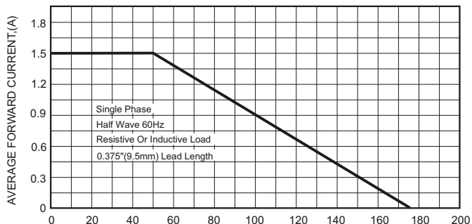
FIG.1-TYPICAL FORWARD CURRENT DERATING CURVE
