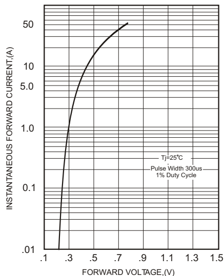
FIG.2-TYPICAL FORWARD CHARACTERISTICS
