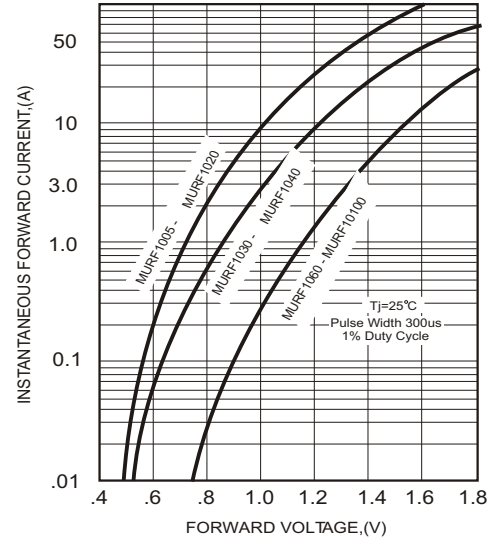
FIG.2-TYPICAL FORWARD CHARACTERISTICS
