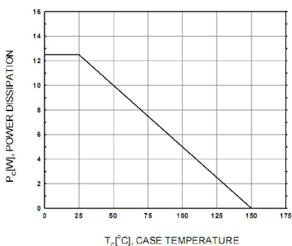
Figure 6. Power Derating
