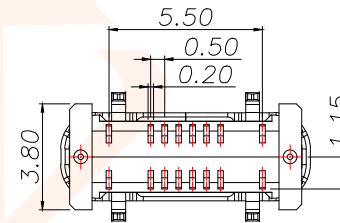
(TOP VIEW) RECOMMENDED P.C.B. LAYOUT (T:0.8mm) TOLERANCE UNSPECIFIED \pm 0.05\text{mm}
