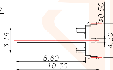
(TOP VIEW) RECOMMENDED P.C.B. LAYOUT (T:0.8mm) TOLERANCE UNSPECIFIED \pm 0.05\text{mm}
