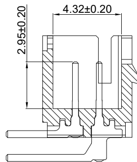
SECTION I-I
