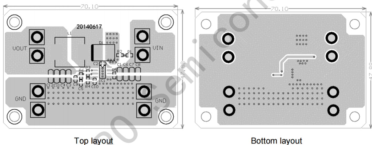
Figure 6: PCB Layout Reference
