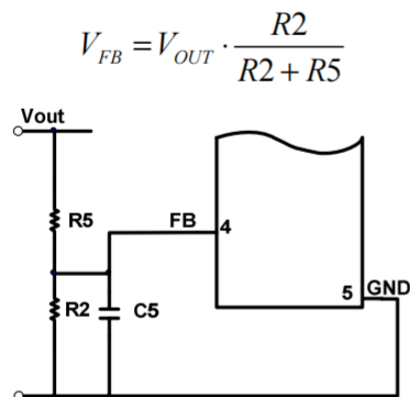
Figure 1: Output Voltage Setup
