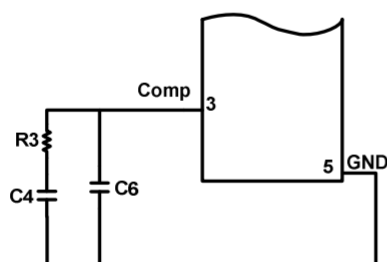
Figure 5: Compensation Loop
