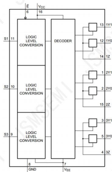
Figure 4. Functional diagram
