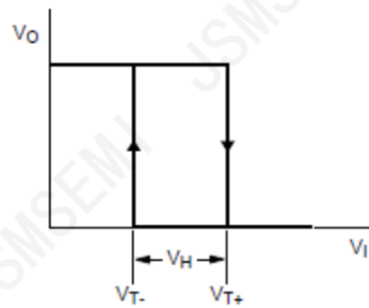
Figure 6. Transfer characteristic
