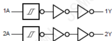
Figure 3. Logic diagram
