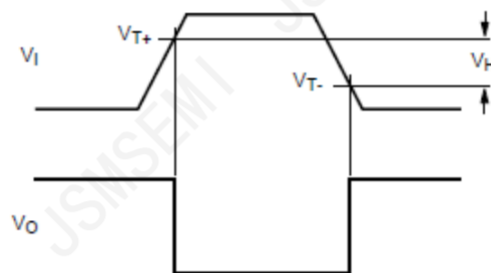
Figure 7. Definition of V_{T+} , V_{T-} and V_H
