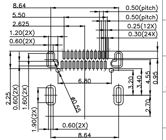
RECOMMENDED P.C.B Dimension Tolerances:±0.05mm
