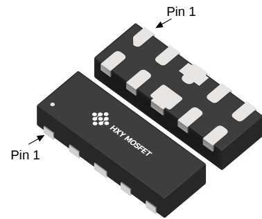
DFN2510-10L
