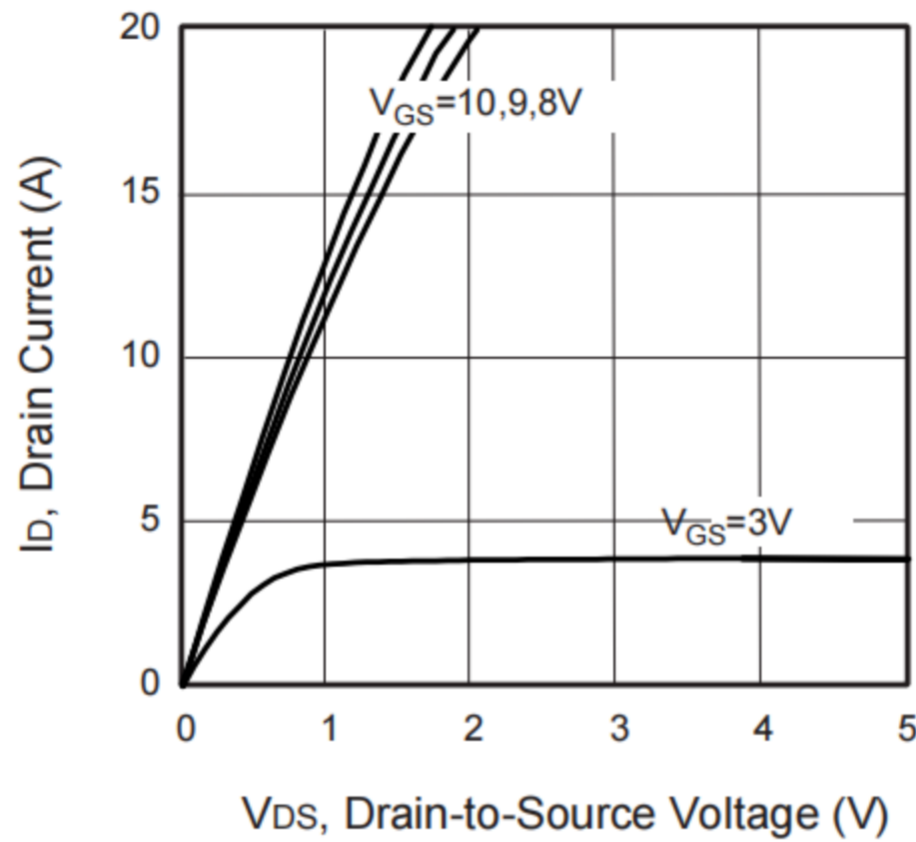
Figure 1. Output Characteristics
