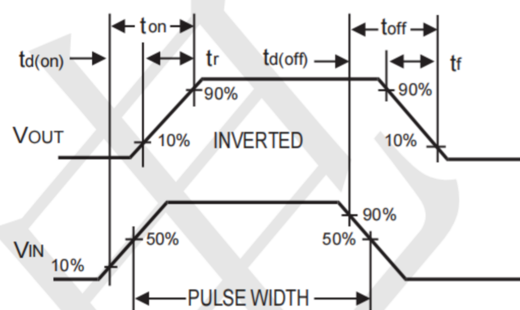
Figure 10. Switching Waveforms
