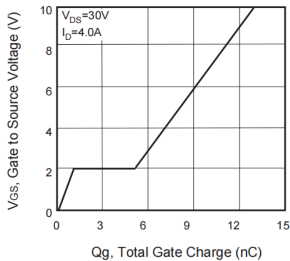
Figure 7. Gate Charge
