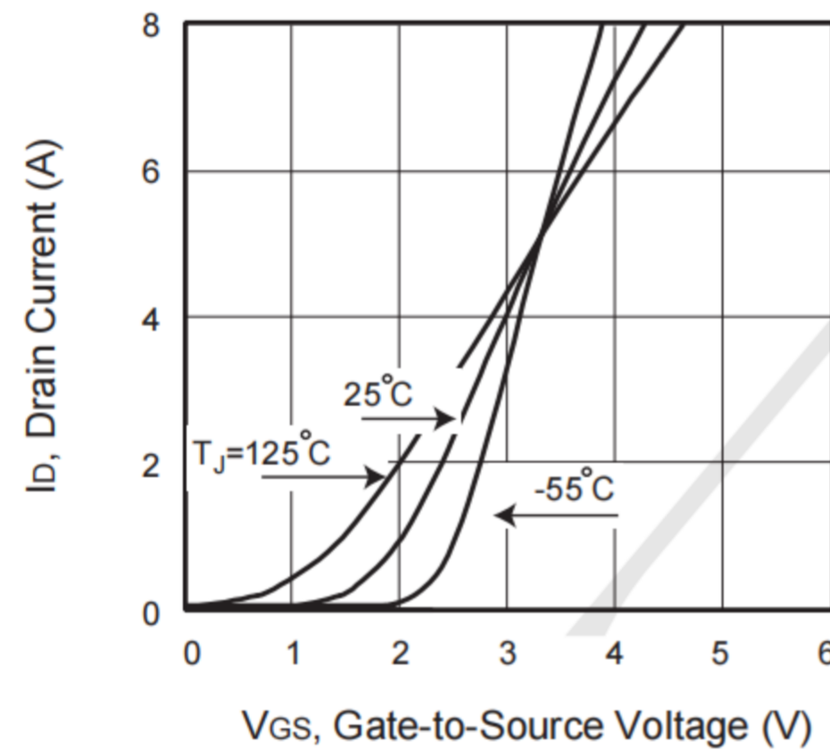
Figure 2. Transfer Characteristics
