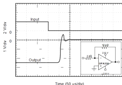
Figure 12. 负过压恢复
