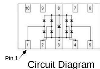
DFN2510-10L (DFN-10(1x2.5))
