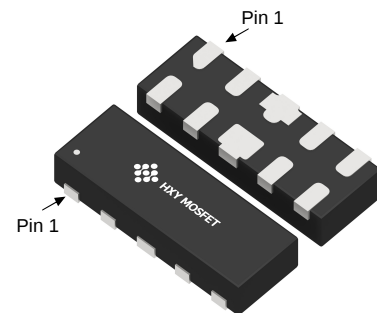
DFN2510-10L (DFN-10(1x2.5))
