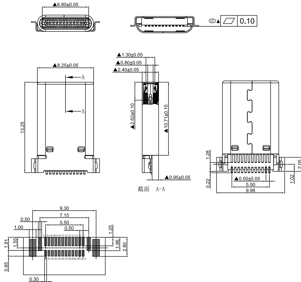
RECOMMENDED PCB LAYOUT GENERAL TOLERANCE \pm 0.05
