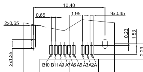
RECOMMENDED P.C.B. LAYOUT TOLERANCE UNSPECIFIED ±0.05mm
