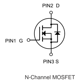
TO-220 (TO-220AB-3)
