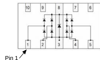
Circuit Diagram
