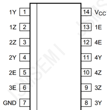
Figure 4. Functional diagram
