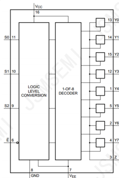
Figure 4. Functional diagram
