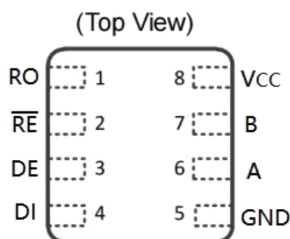
DFN-8 3*3/DFN-8 2*2
