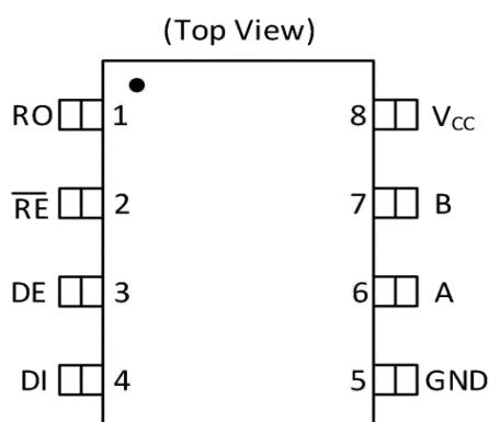
SOP-8
