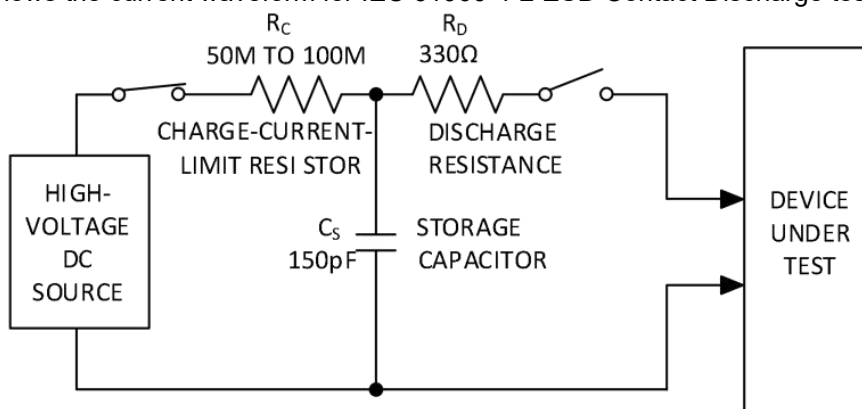
Figure 10c. IEC 61000-4-2 ESD Test Model
