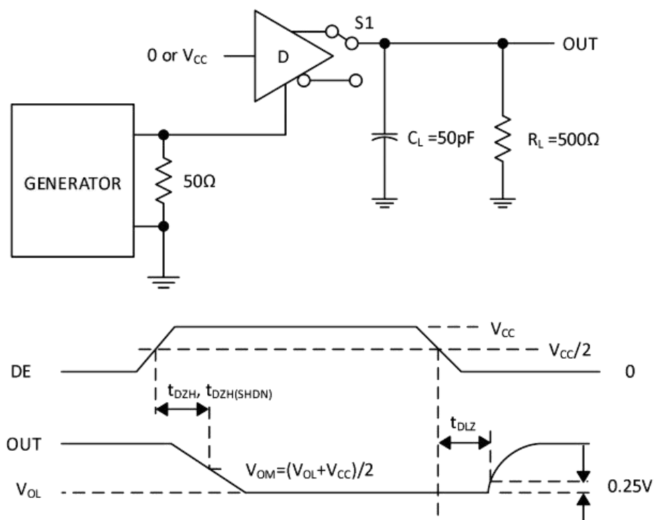
Figure 5. Driver Enable and Disable Times ( t_{DZL} , t_{DLZ} , t_{DLZ(SHDN)} , t_{DZL(SHDN)} )
