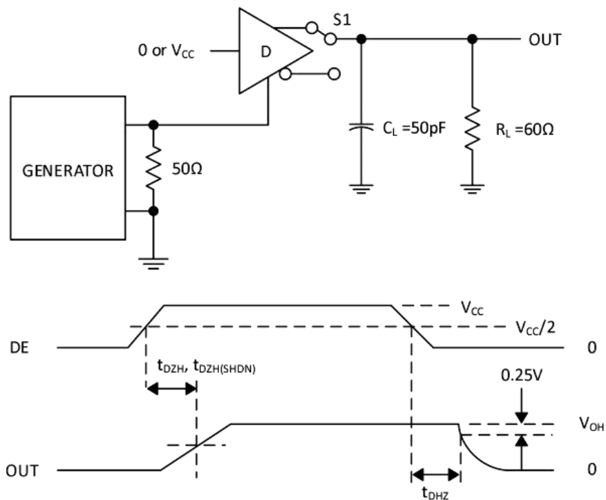
Figure 4. Driver Enable and Disable Times ( t_{DZH} , t_{DZH(SHDN)} , t_{DZL} , t_{DZL(SHDN)} )
