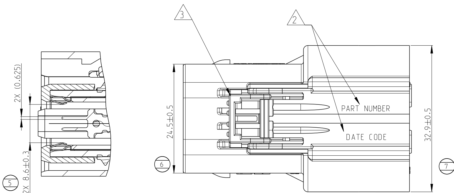
SECTION E-E SCALE 2:1
