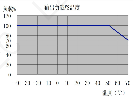
工作温度降额曲线图 Operating Temperature Derating Curve
