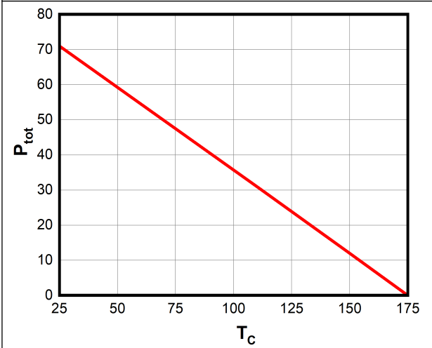
Figure 6. Power Derating
