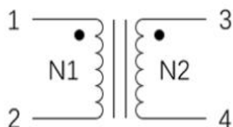
绕线结构表 Winding Structure Diagram
