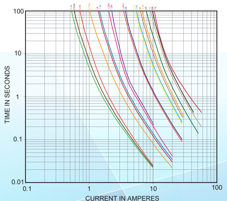
Average Time-Current Curve
