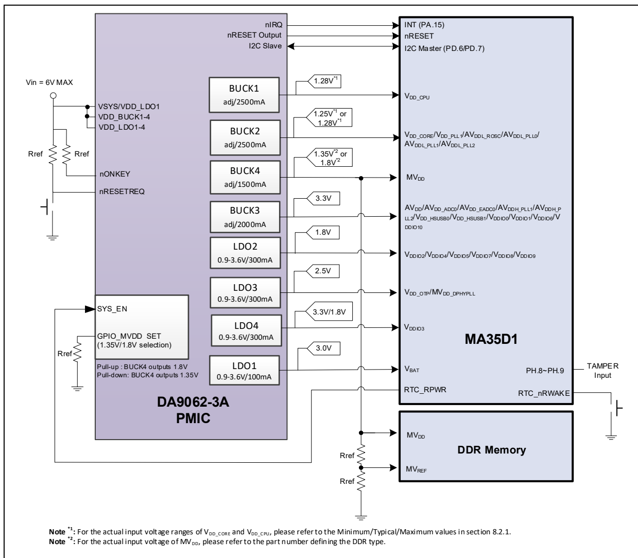
Figure 8-2 System Power Scheme Diagram
