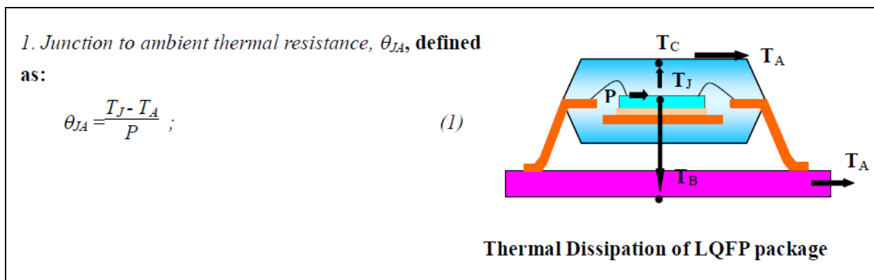
Figure 9-4 Junction to Ambient Thermal Resistance
