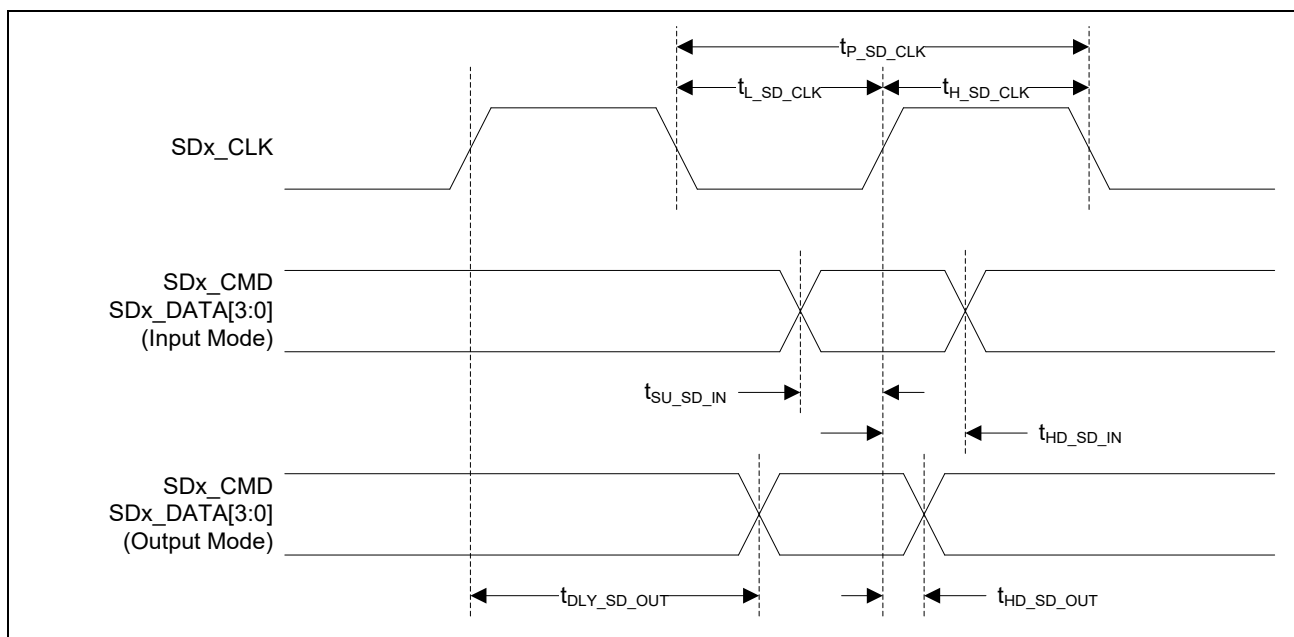
Figure 8-23 SD High-Speed Mode Timing Diagram
