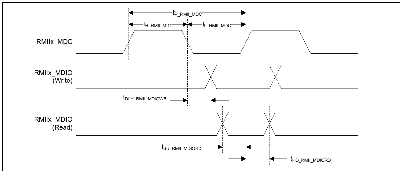
Figure 8-19 Ethernet PHY Management Interface Timing Diagram
