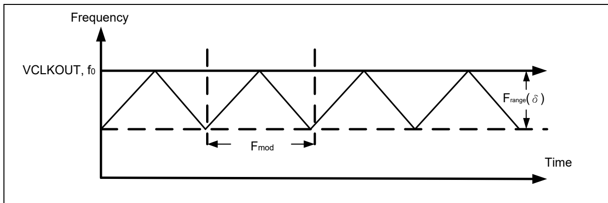
Figure 6-16 Advanced PLL Down Spreading in Spectrum Mode
