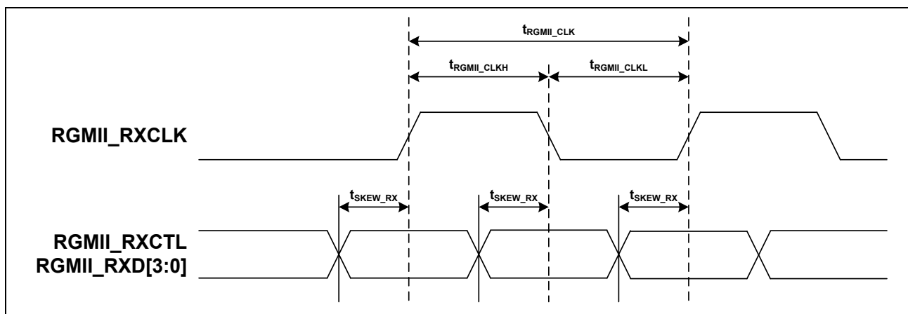
Figure 8-18 RGMII Receive Timing Diagram
