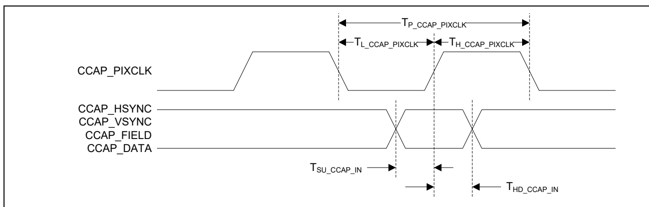
Figure 8-26 CCAP Timing Diagram
