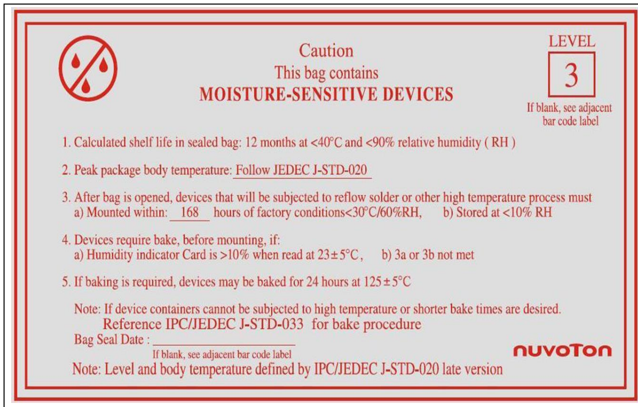
Figure 9-8 Cautions for PKG Baking
