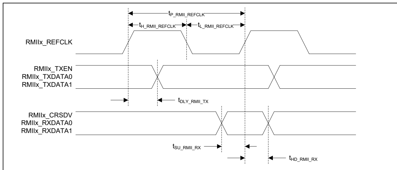
Figure 8-16 RMII Interface Timing Diagram
