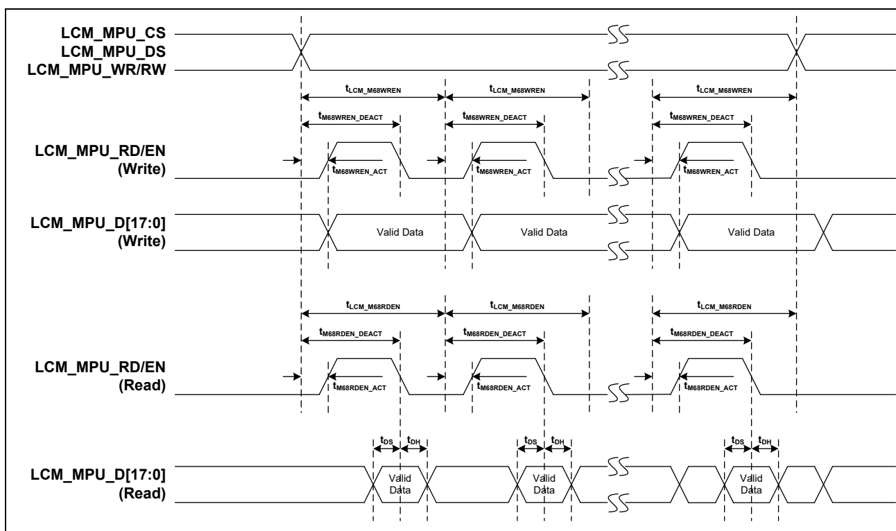
Figure 8-29 LCD MPU M68 Mode Timing Diagram
