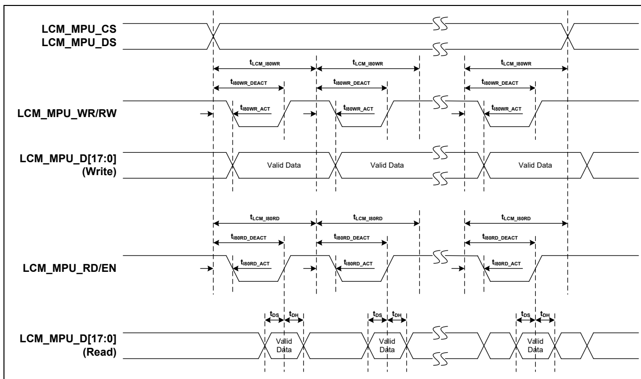
Figure 8-28 LCD MPU I80 Mode Timing Diagram
