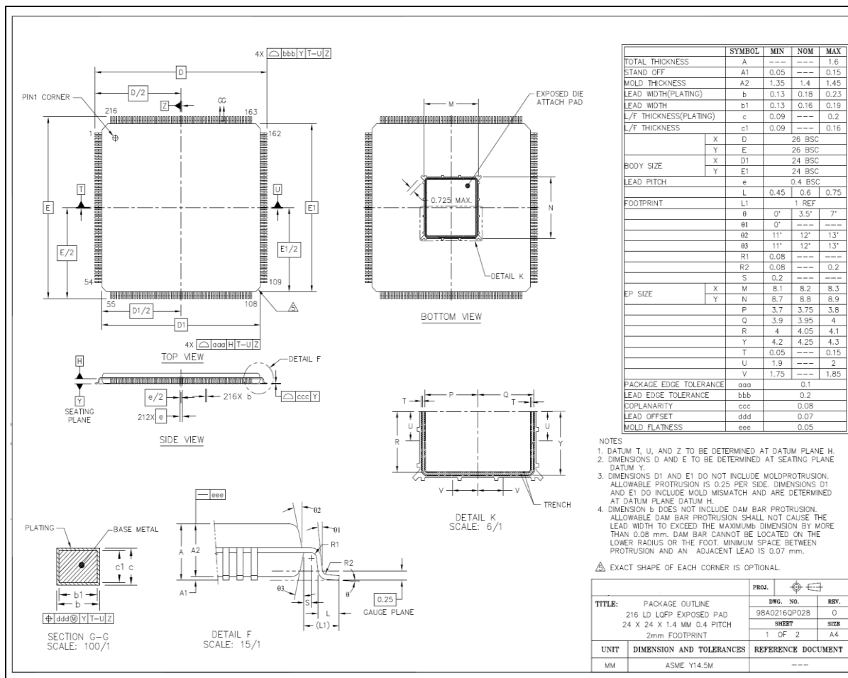
Figure 9-1 LQFP-EP 216-Pin Package Demension
