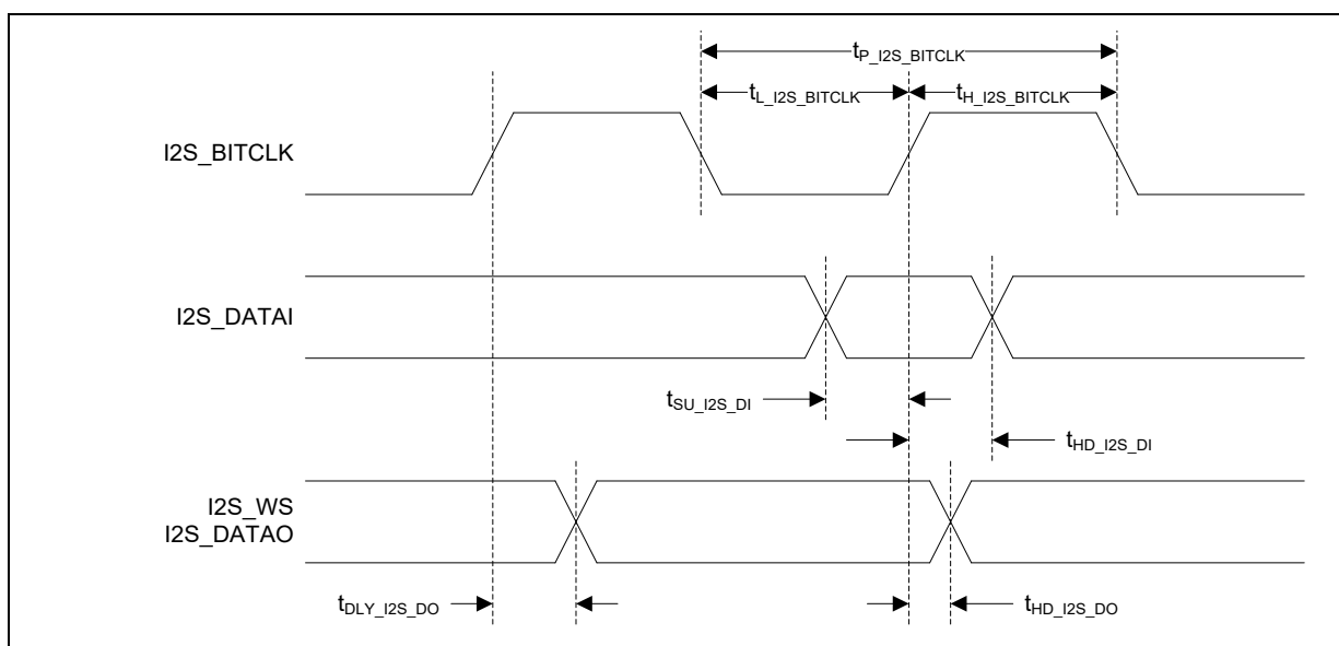
Figure 8-15 I 2 S Timing Diagram
