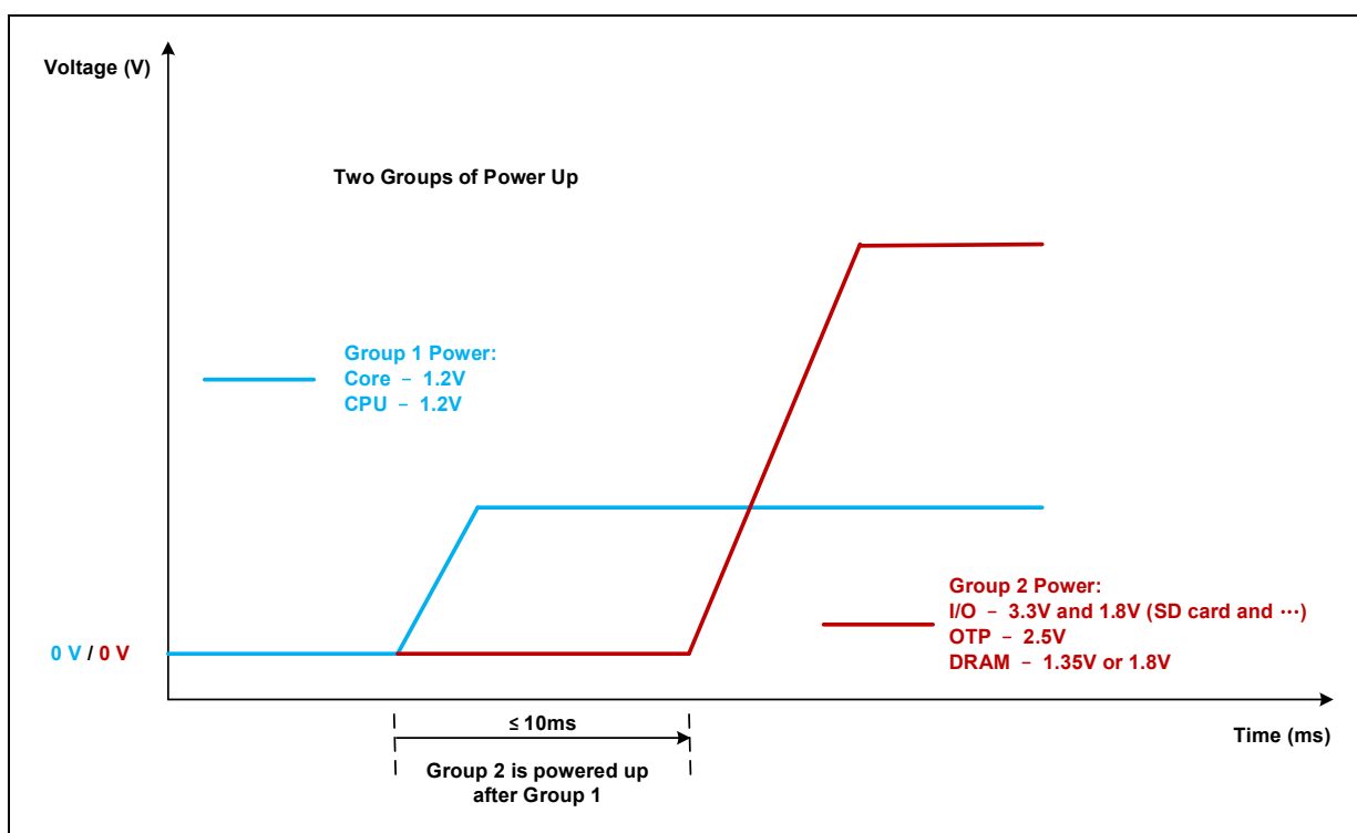
Figure 8-8 Power Sequence and nRESET
