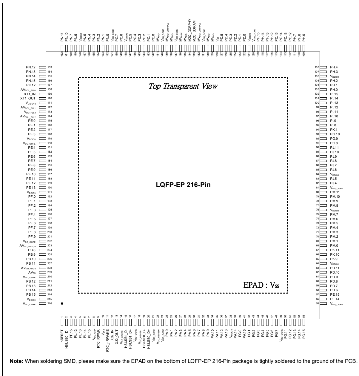
Figure 4-1 NuMicro MA35D1 Series LQFP-EP 216-Pin Pinout Diagram
