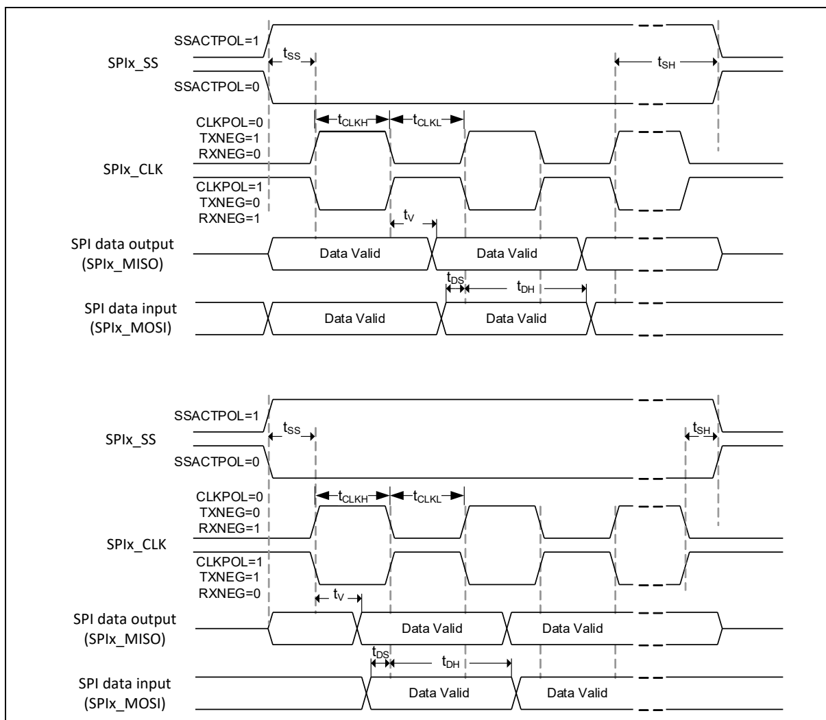
Figure 8-12 SPI Slave Mode Timing Diagram
