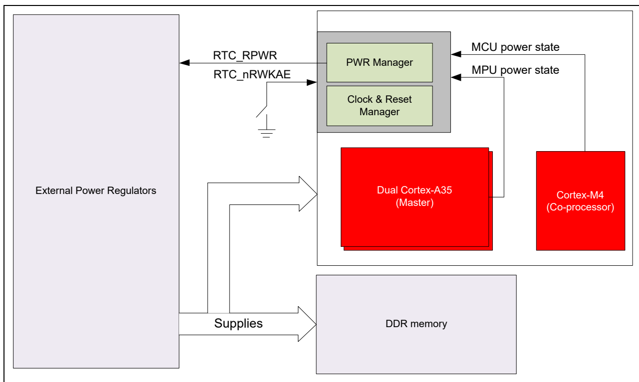
Figure 8-3 System Power Management Architecture
