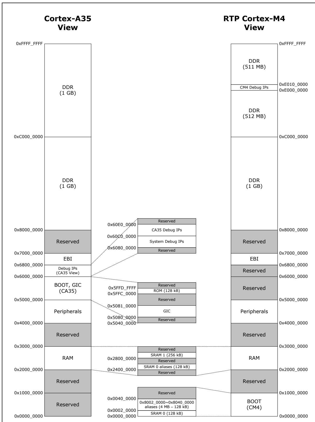
Figure 6-6 MA35D1 System Memory Map Diagram
