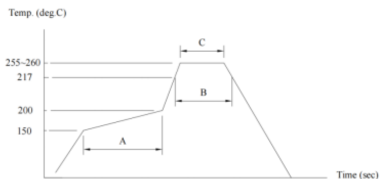
Figure 6 Reflow Profile
