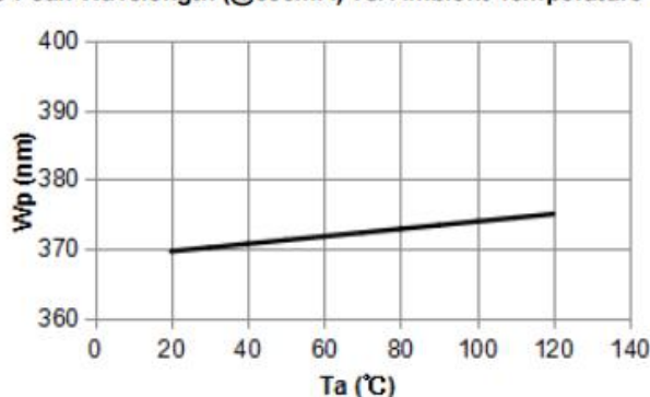
Fig.5-Peak Wavelength (@500mA) vs. Ambient Temperature
